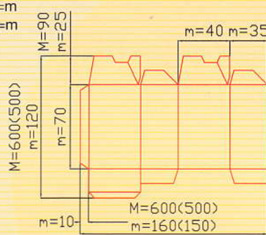
勾底盒 Crash-Lock Bottom Box
