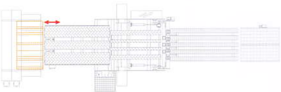
Mod. 15.25 - mobile with shuttle car
