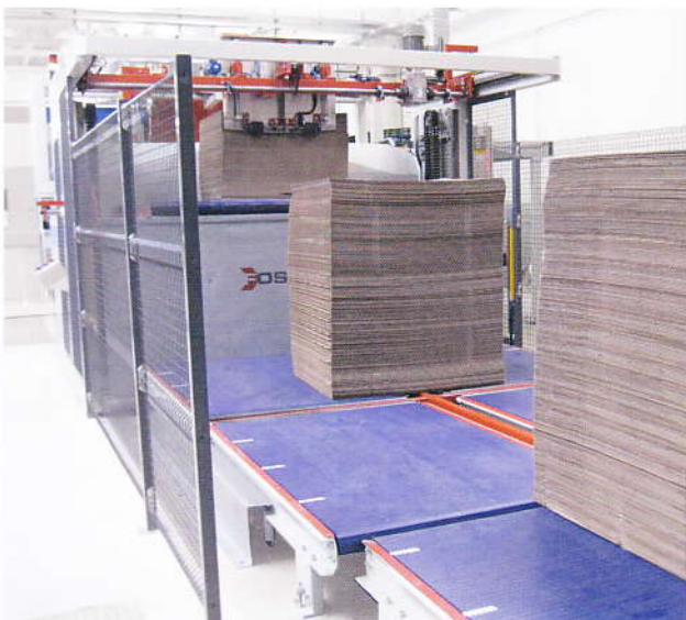
Modular belt conveyors with 90°/180° turning cross
